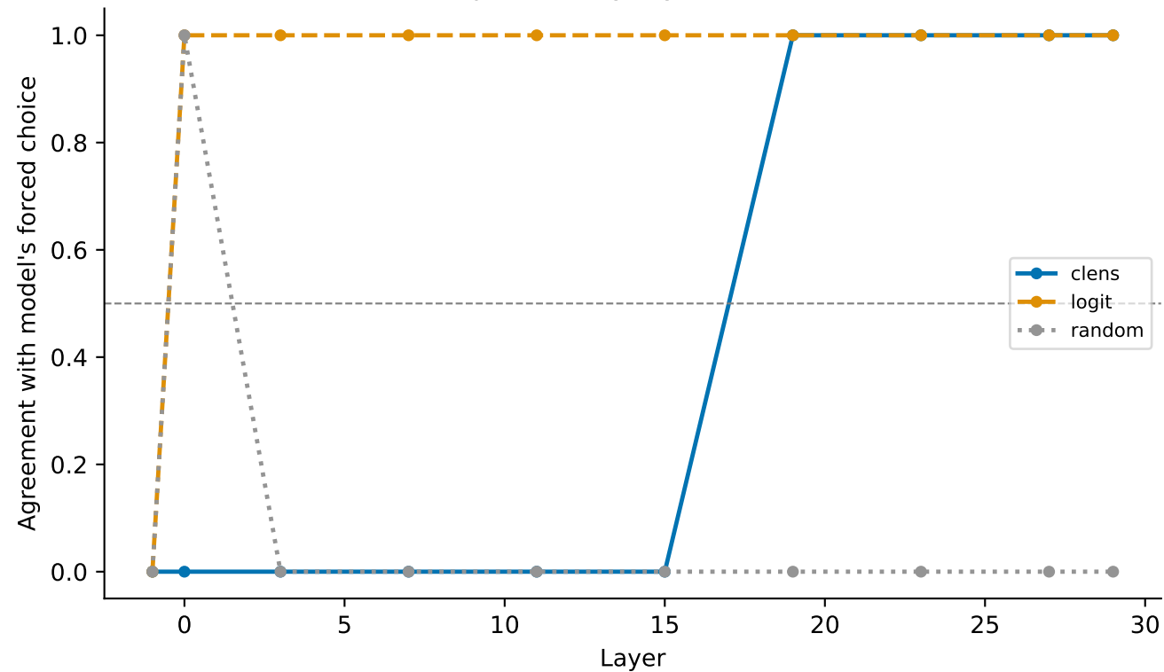
V3 taint disposition by layer — starcoder2-3b
