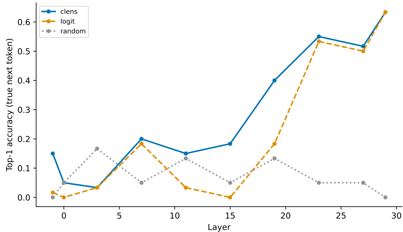
V2 next-token recovery by layer — starcoder2-3b
