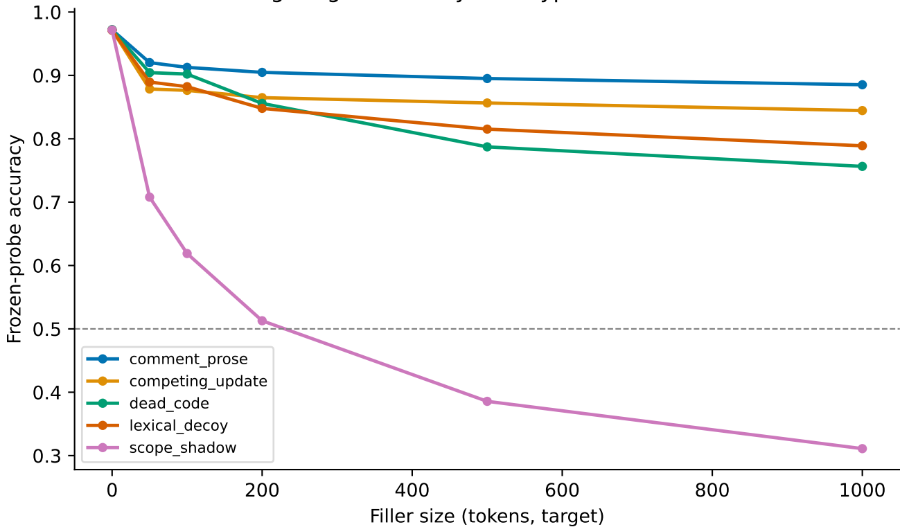
binding: degradation by filler type — starcoder2-3b
