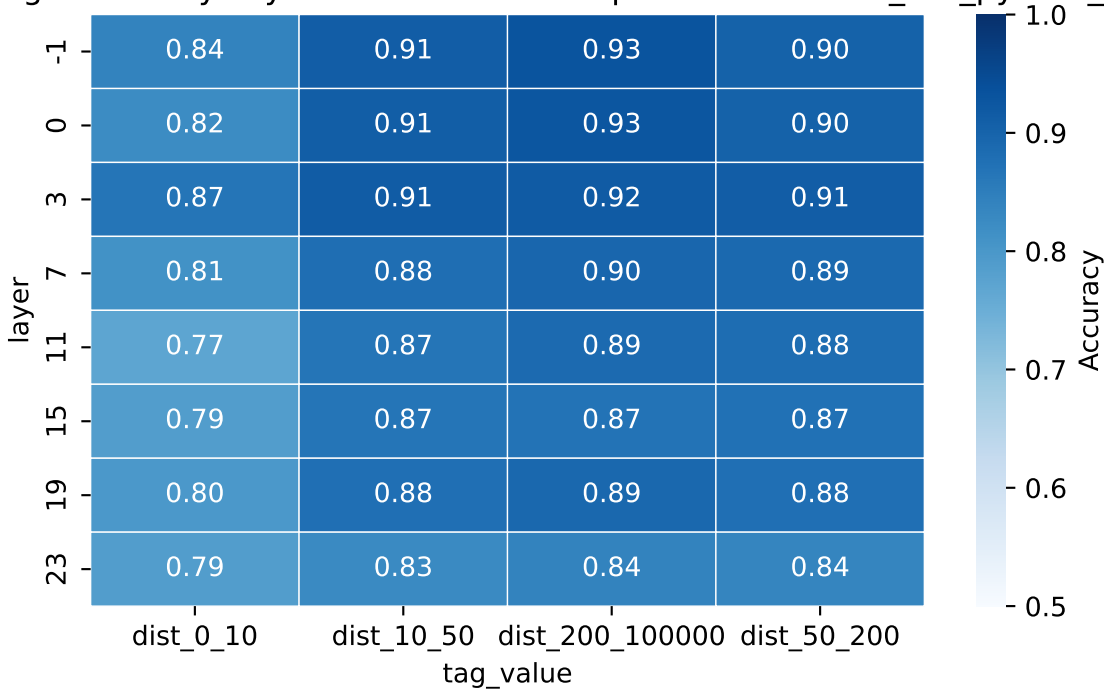
Def-use edge accuracy: layer × distance — deepseek-coder-1.3b_csn_python_200
