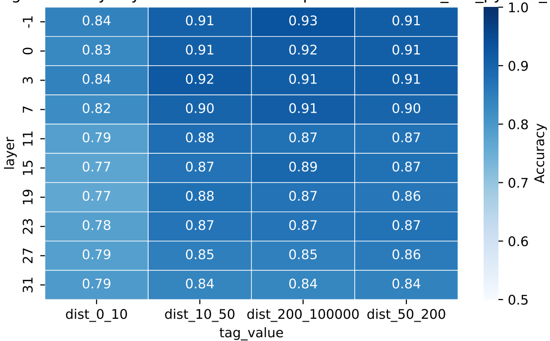
Def-use edge accuracy: layer × distance — deepseek-coder-6.7b_csn_python_200
