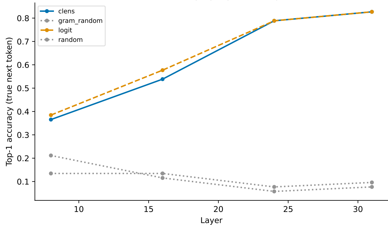
E11 V2: next-token recovery by layer — deepseek-coder-6.7b
