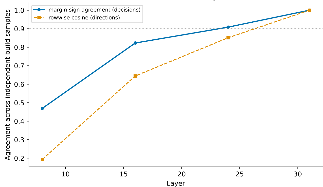
E11: lens stability across seeds — deepseek-coder-6.7b (dotted line = the 0.90 usability threshold)
