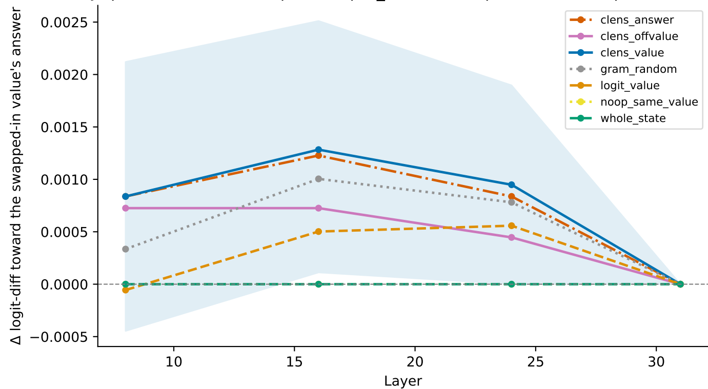
E11: J-space coordinate swap at the pre_def (control position) — deepseek-coder-6.7b
