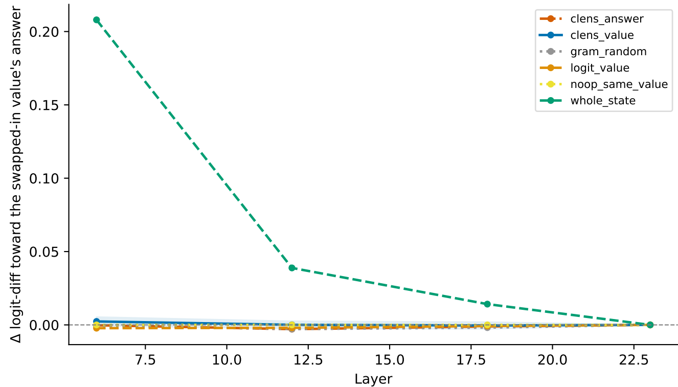
E11: J-space coordinate swap at the marked use — deepseek-coder-1.3b
