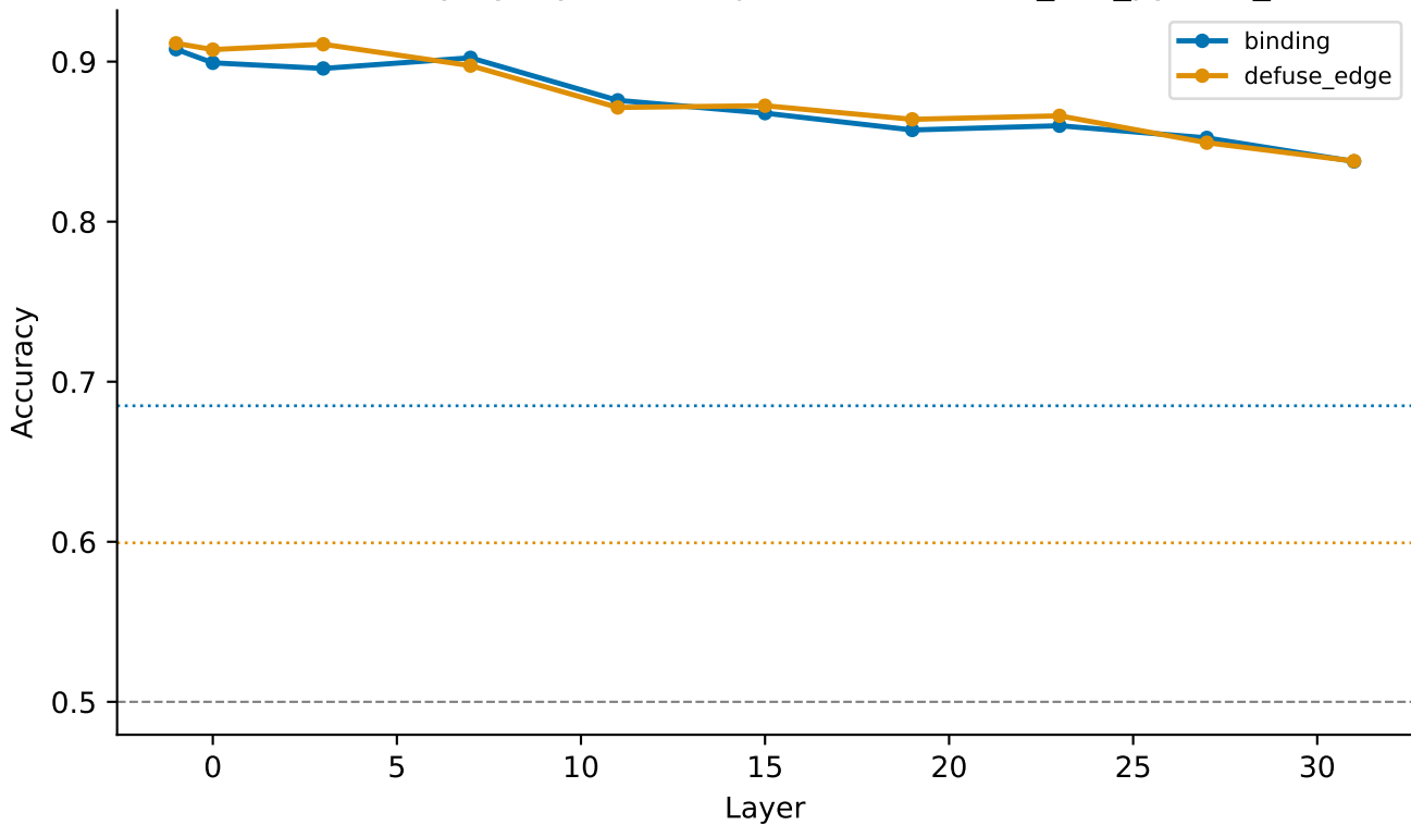
Probe accuracy by layer — deepseek-coder-6.7b_csn_python_200
