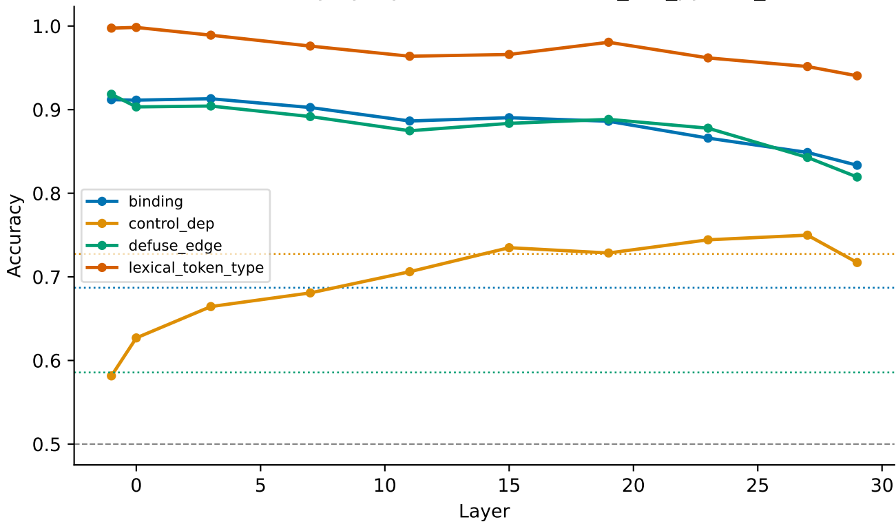
Probe accuracy by layer — starcoder2-3b_csn_python_200
