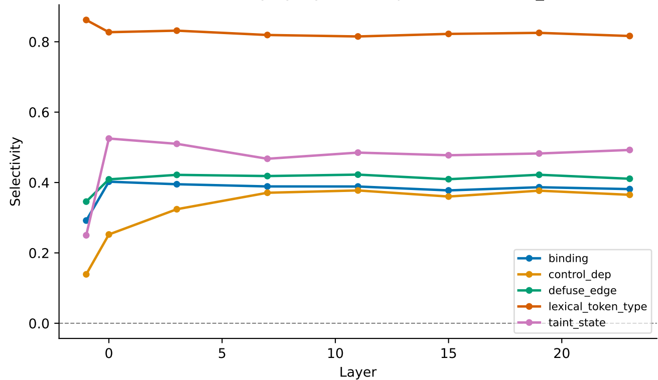
Probe selectivity by layer — deepseek-coder-1.3b_core
