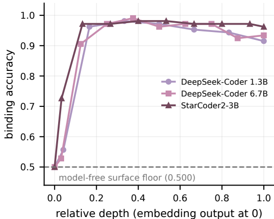
(a) Binding is built in context
