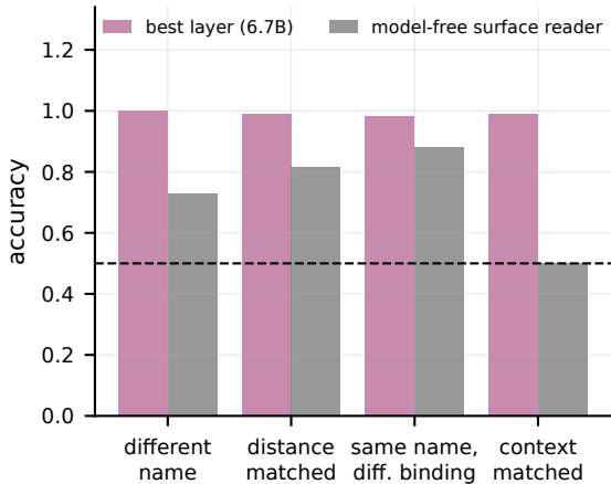
(b) Only one stratum has a floor at chance
