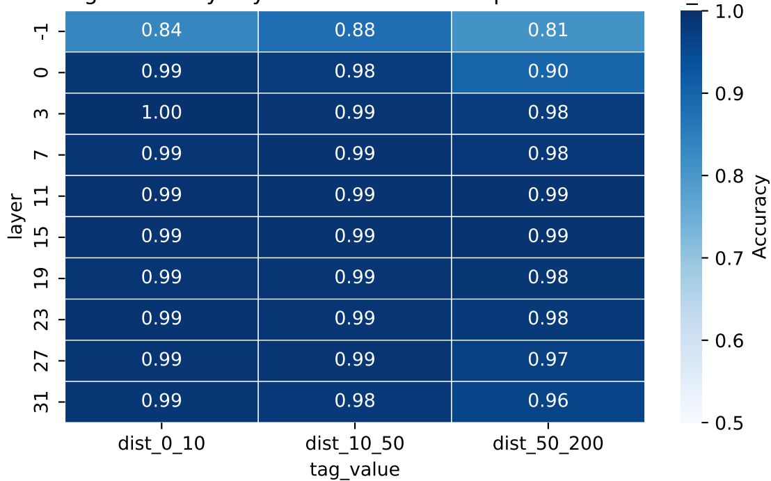
Def-use edge accuracy: layer x distance — deepseek-coder-6.7b_core
