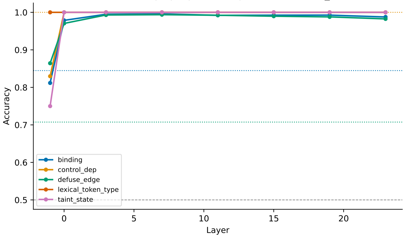
Probe accuracy by layer — deepseek-coder-1.3b_core
