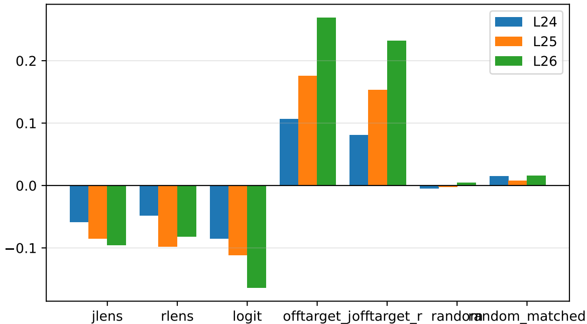
starcode2-3b: erasing the lens read direction
