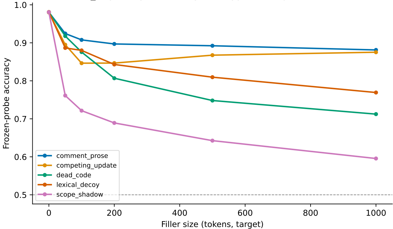
defuse_edge: degradation by filler type — deepseek-coder-6.7b
