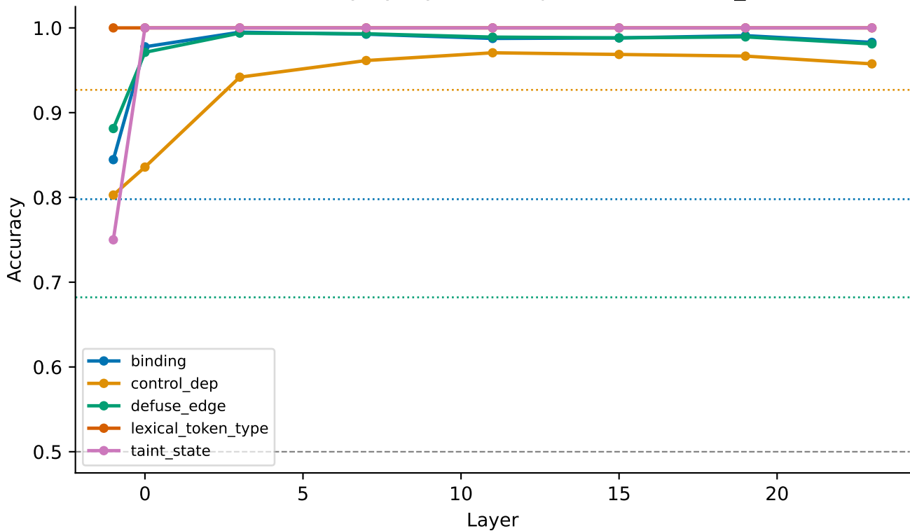
Probe accuracy by layer — deepseek-coder-1.3b_core
