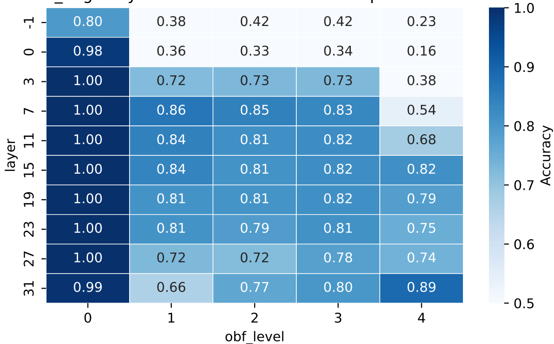
defuse_edge: layer × obfuscation level — deepseek-coder-6.7b
