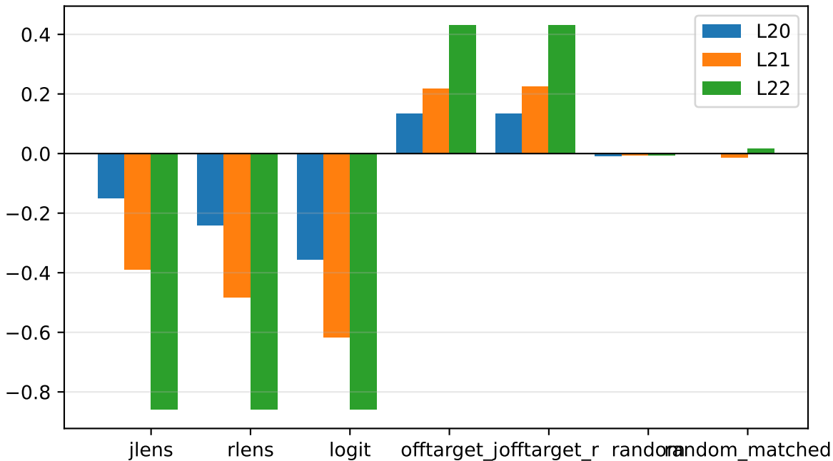
deepseek-coder-1.3b: erasing the lens read direction
