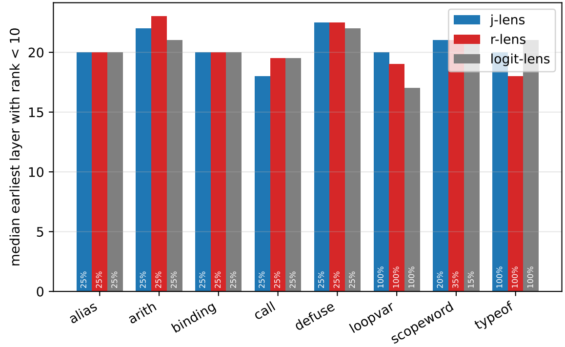
starcoder2-3b-paperminimal: where the concept first appears (bar label = share of items that ever reach top 10)
