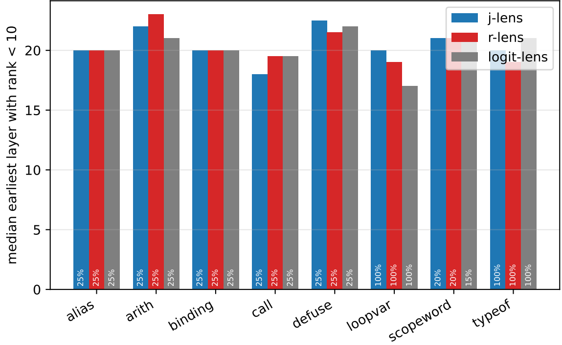
starcoder2-3b: where the concept first appears (bar label = share of items that ever reach top 10)
