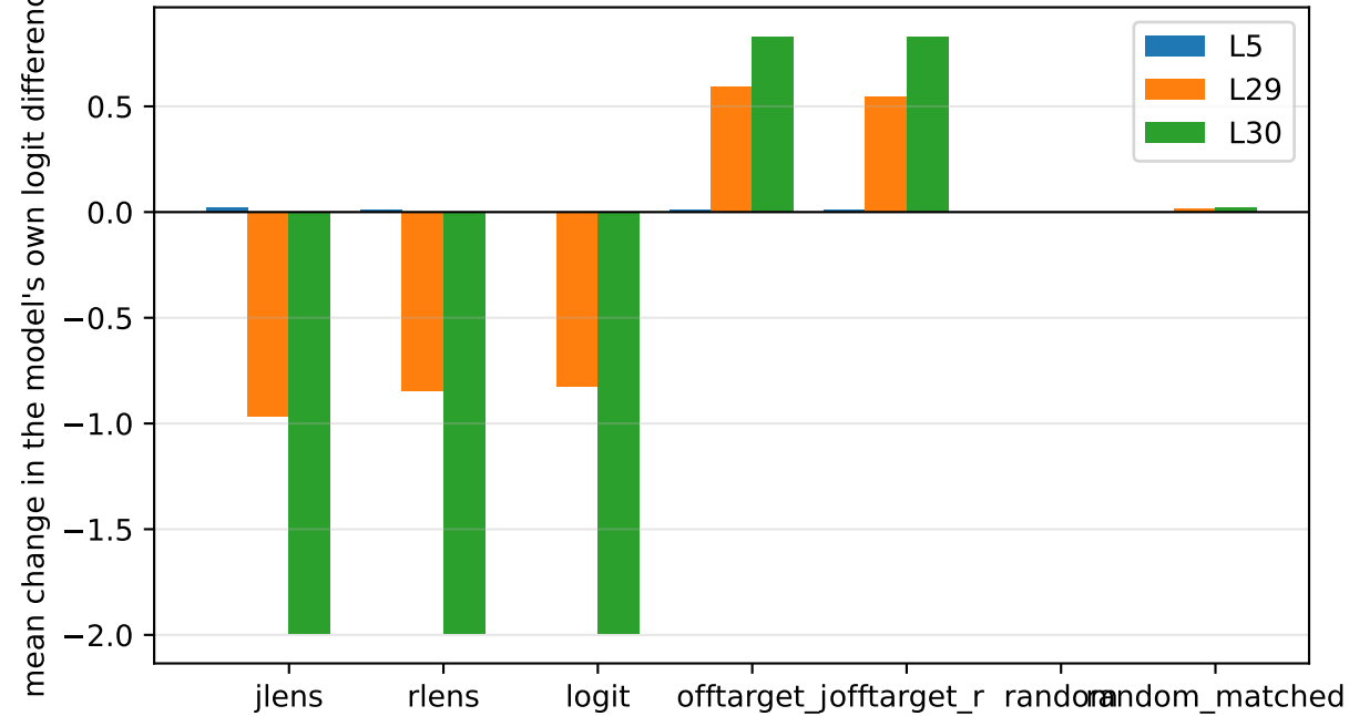
deepseek-coder-6.7b: erasing the lens read direction
