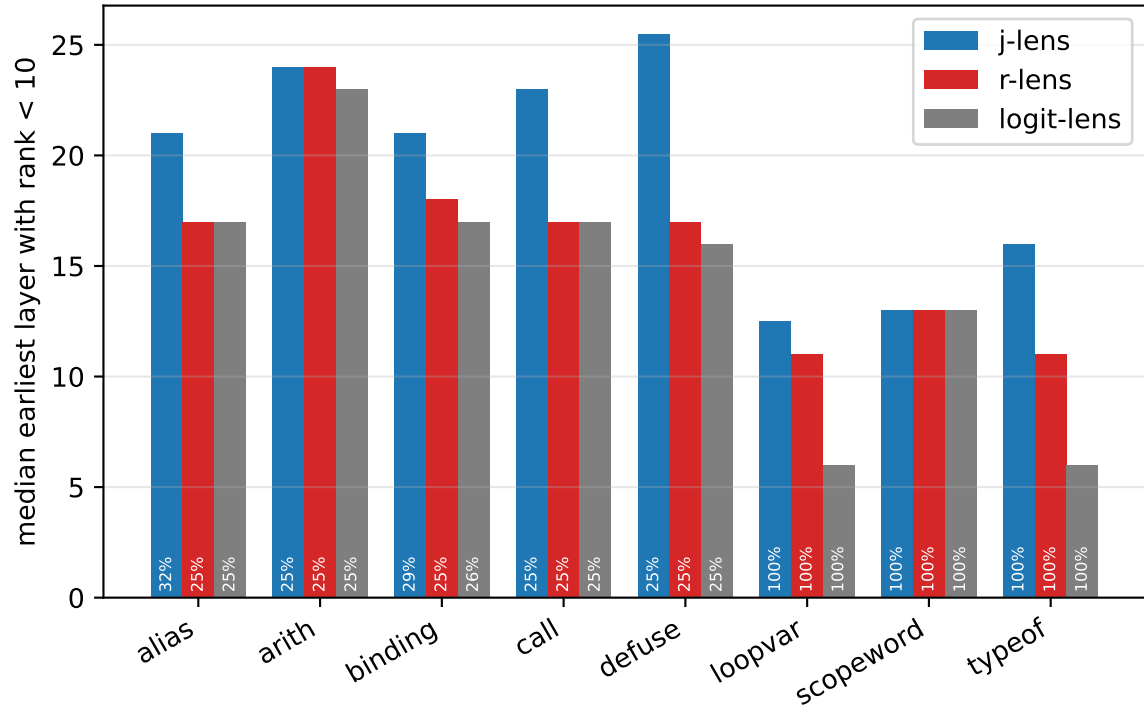
deepseek-coder-6.7b: where the concept first appears (bar label = share of items that ever reach top 10)
