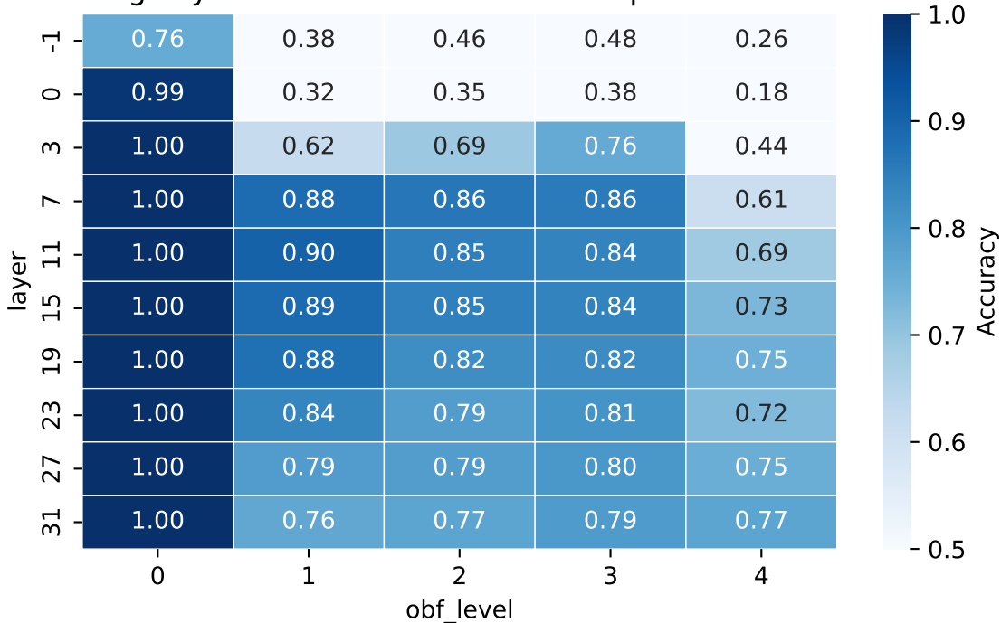
binding: layer × obfuscation level — deepseek-coder-6.7b
