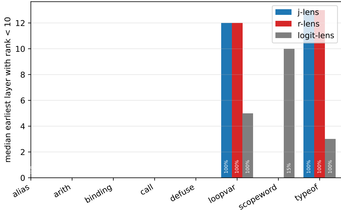
deepseek-coder-1.3b: where the concept first appears (bar label = share of items that ever reach top 10)
