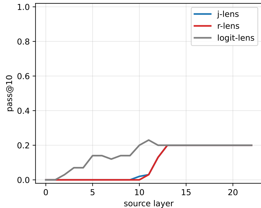
deepseek-coder-1.3b: what the lenses surface across layers all items (n=100)
