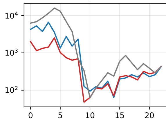
scopeword
