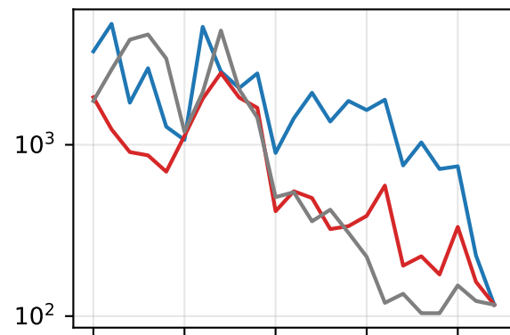
call
