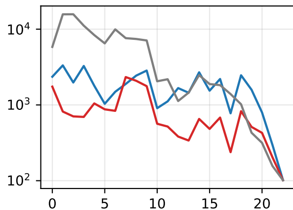
defuse
