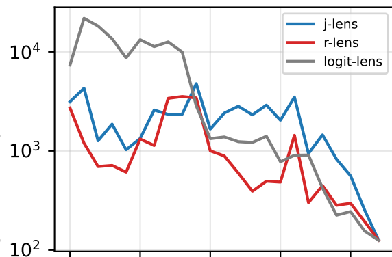
alias
