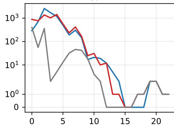
typeof
