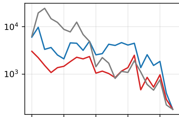
arith
