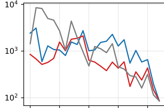
binding
