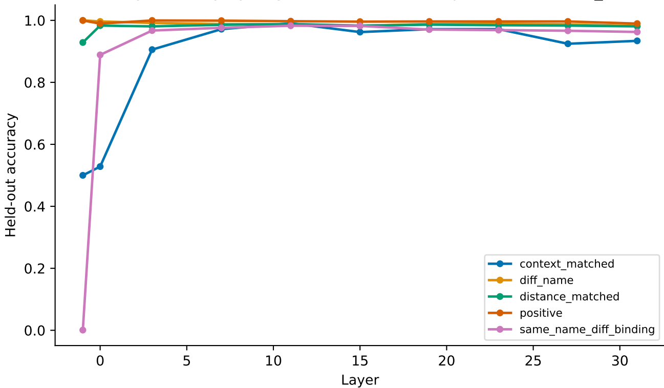
Binding accuracy by negative stratum — deepseek-coder-6.7b_core
