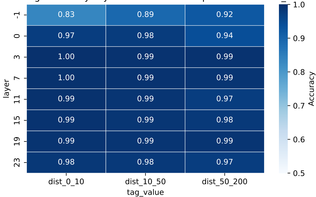
Def-use edge accuracy: layer × distance — deepseek-coder-1.3b_core
