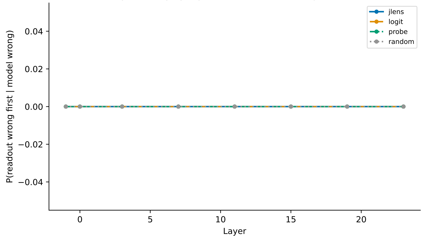
E10-2 early warning by layer and readout — deepseek-coder-1.3b
