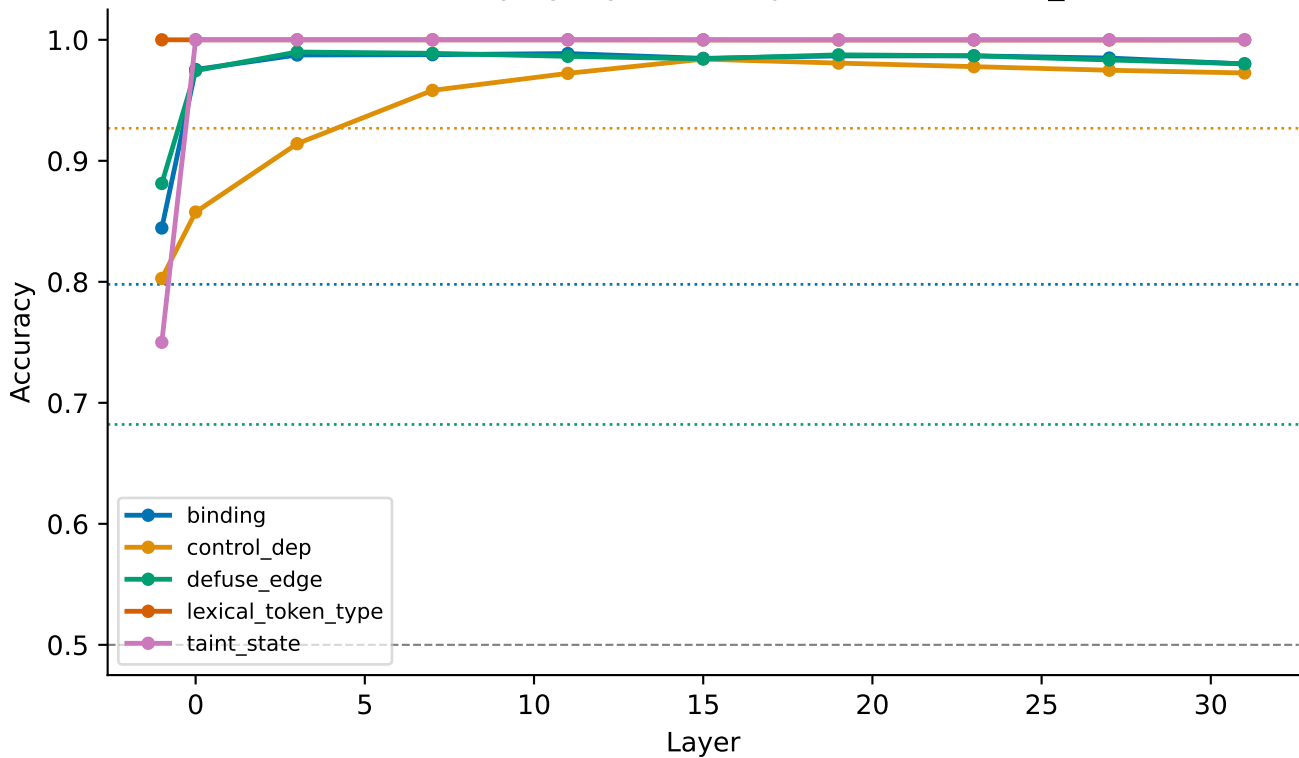
Probe accuracy by layer — deepseek-coder-6.7b_core
