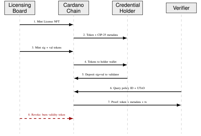
Fig. 7. Sequence diagram: credential lifecycle from issuance through verification and revocation.
