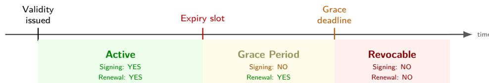
Figure 4.7: Dues enforcement timeline. The active period allows both signing and renewal. The grace period blocks signing but allows dues payment. After the grace deadline, the authority can revoke.
