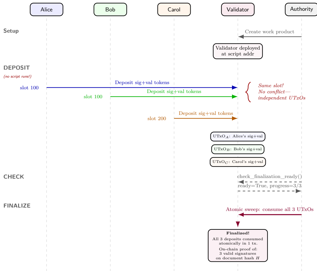
Figure 4.6: Sequence diagram showing the Deposit → FINALIZE flow with three signers. Alice and Bob deposit in the same slot without conflict because each creates an independent UTxO—no validator script runs during deposits. Carol deposits later. The authority then atomically sweeps all three UTxOs in a single finalization transaction, which is the point where the validator executes and enforces all rules.
