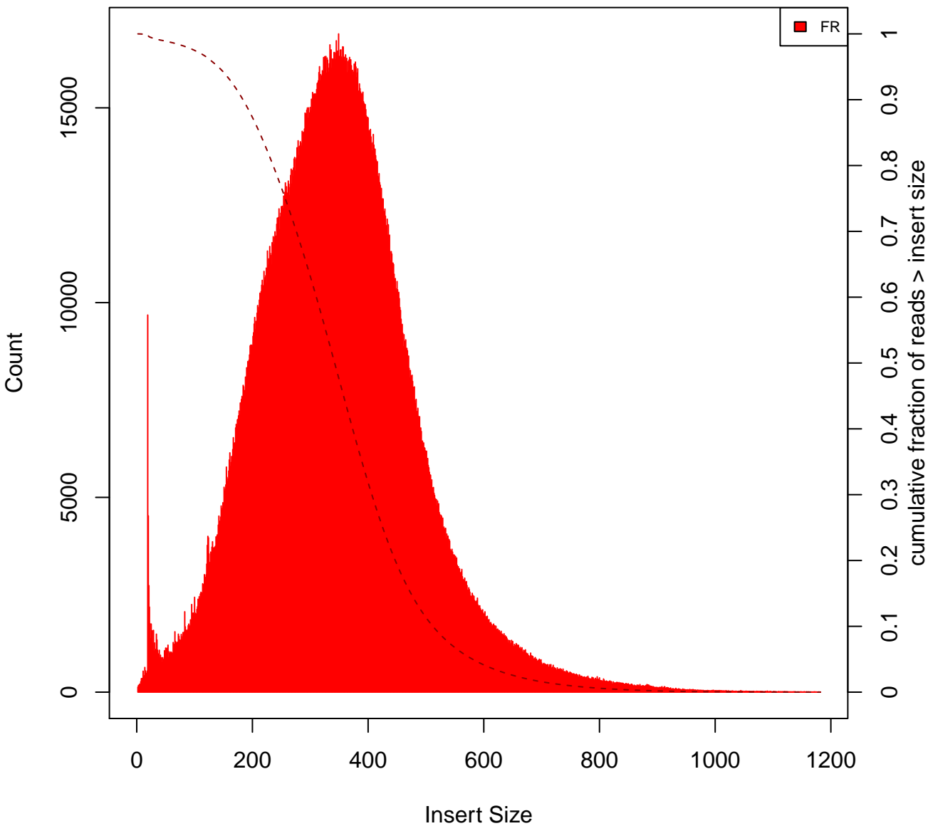
Insert Size Histogram for All_Reads in file KP076.sorted.bam
