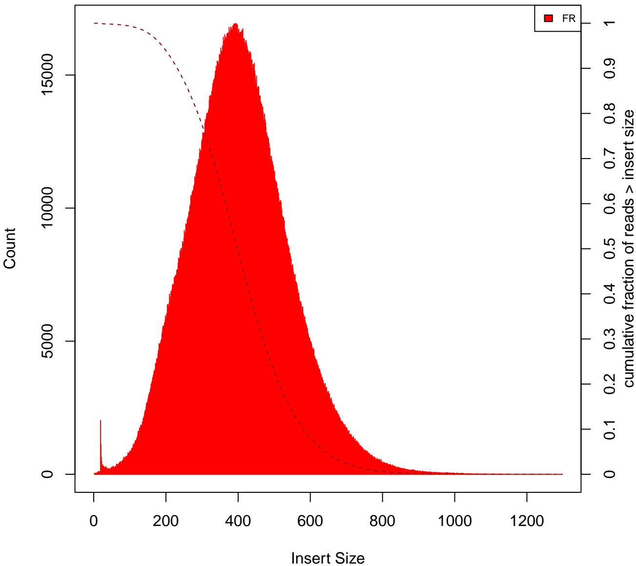
Insert Size Histogram for All_Reads in file KP014.sorted.bam
