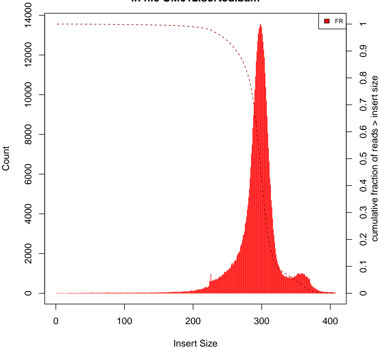
Insert Size Histogram for All_Reads in file OM012.sorted.bam
