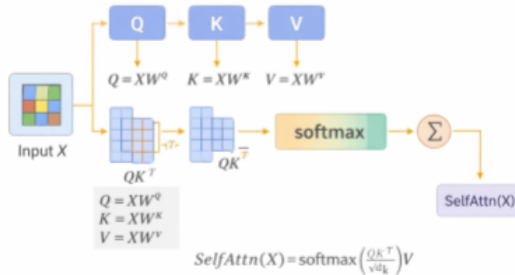
Fig 4: Self- Attention Mechanism
