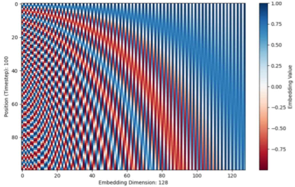
Fig 9: positional encoding heatmap
