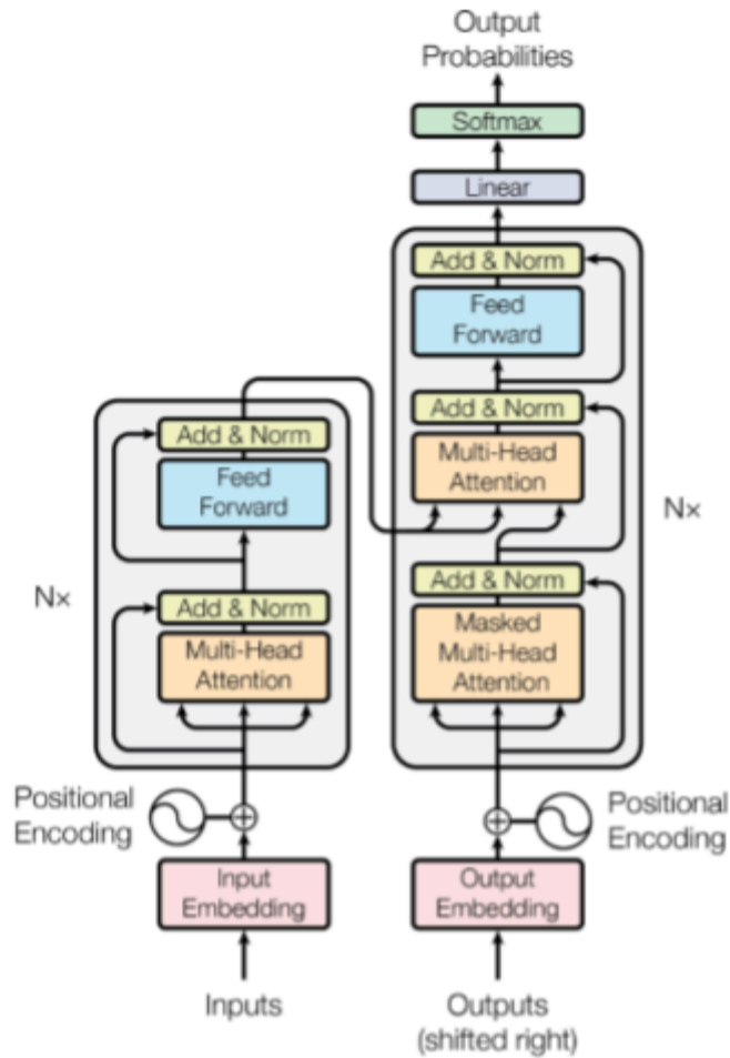
Fig 7 : The Transformer - model architecture. Figure adapted from Vaswani et al. , "Attention Is All You Need" (2017)."
