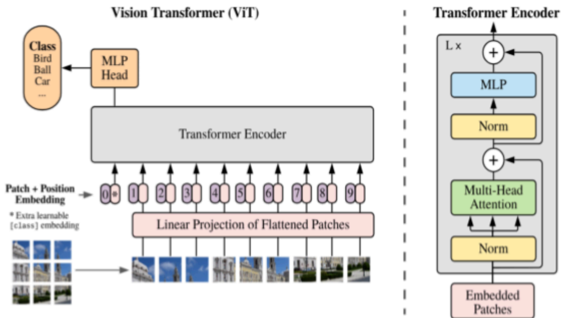
Fig 8: Model overview. We split an image into fixed-size patches, linearly embed each of them, add position embeddings, and feed the resulting sequence of vectors to a standard Transformer encoder. In order to perform classification, we use the standard approach of adding an extra learnable "classification token" to the sequence. The illustration of the Transformer encoder was inspired by Vaswani et al. (2017).
