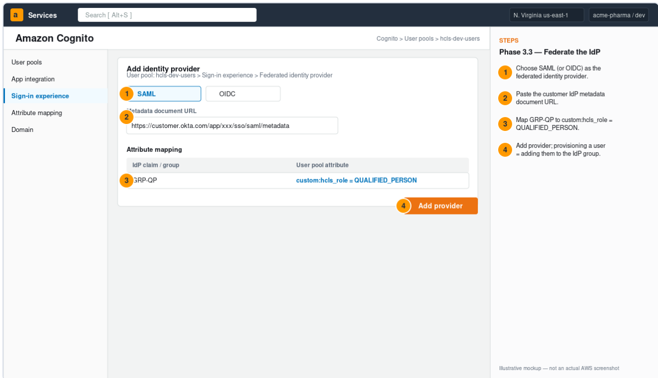
Figure 3. Cognito → Sign-in experience: map GRP-QP → QUALIFIED_PERSON (illustrative mockup).
