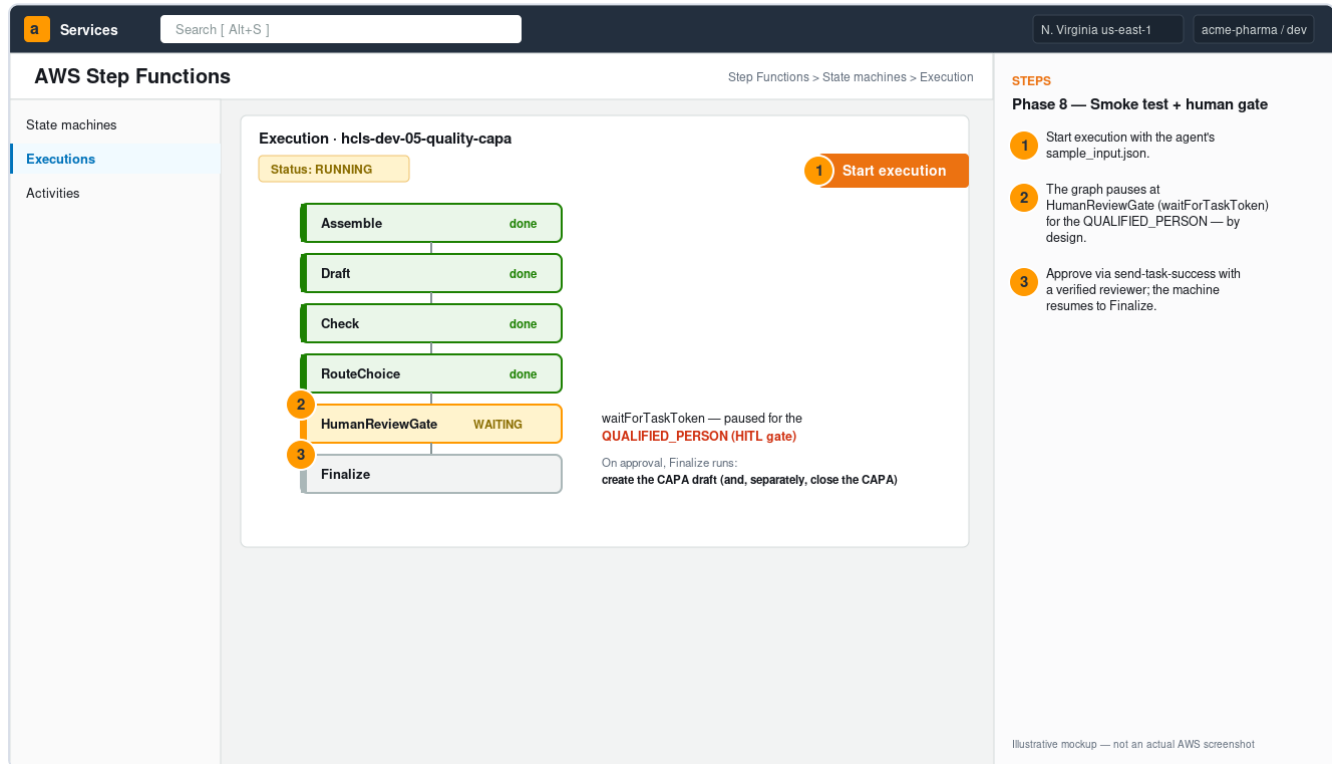
Figure 6. Execution paused at HumanReviewGate for the QUALIFIED_PERSON (illustrative mockup).
