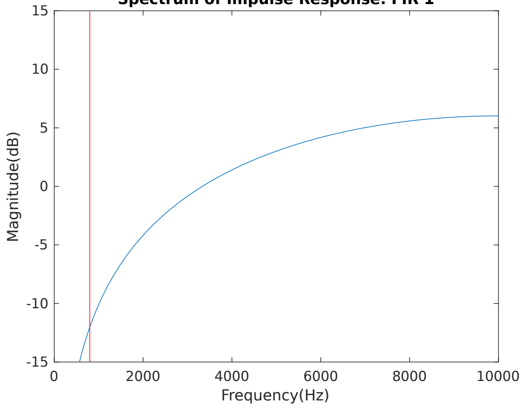
Spectrum of Impulse Response: FIR 1
