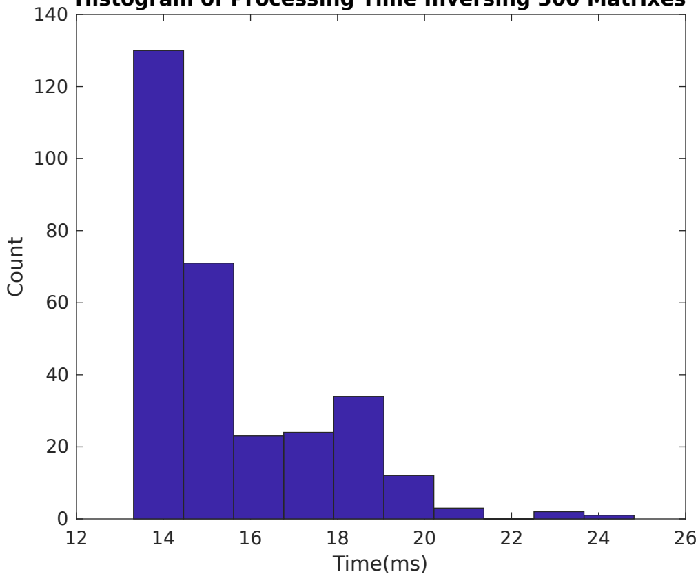
Histogram of Processing Time Inversing 300 Matrixes
