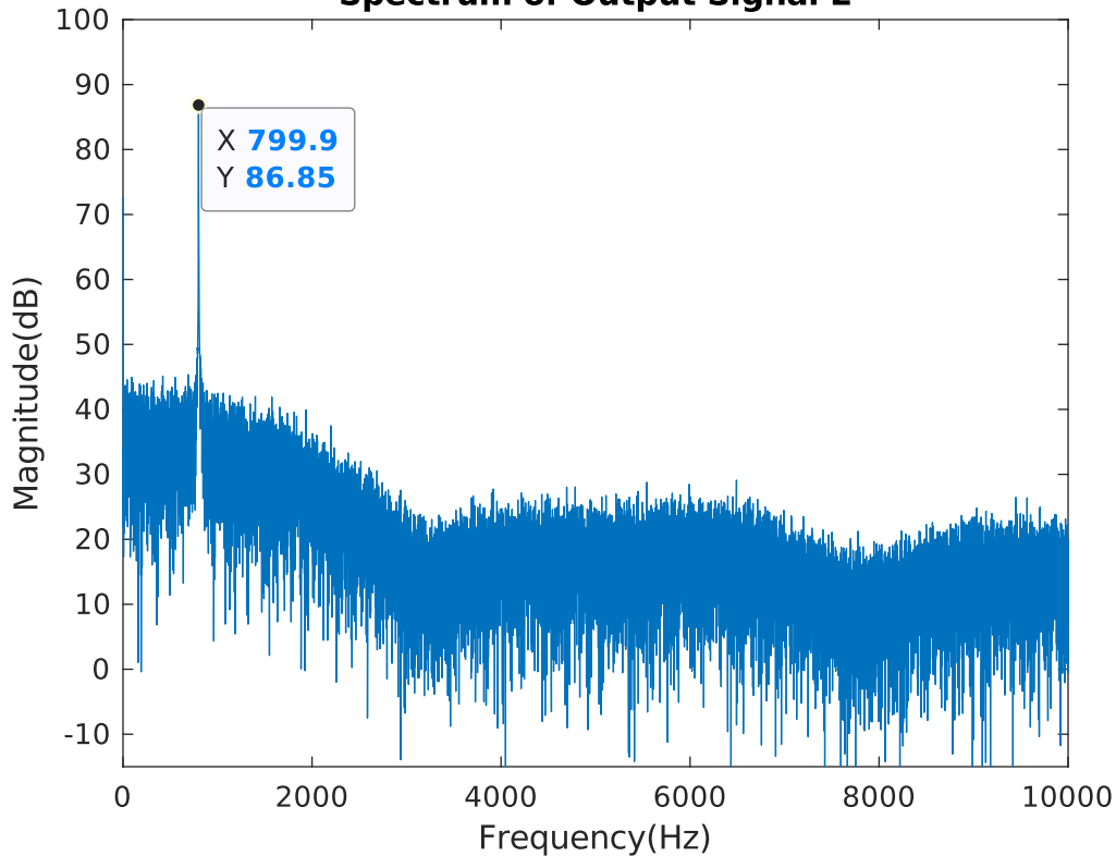
Spectrum of Output Signal 2
