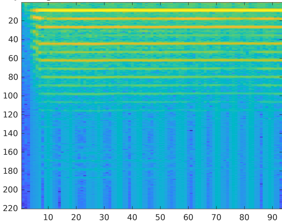
Spectrogram of sound.flute, Frame len. 10ms, Raw matrix
