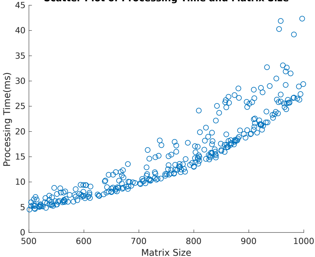
Scatter Plot of Processing Time and Matrix Size
