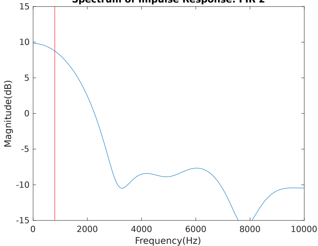
Spectrum of Impulse Response: FIR 2
