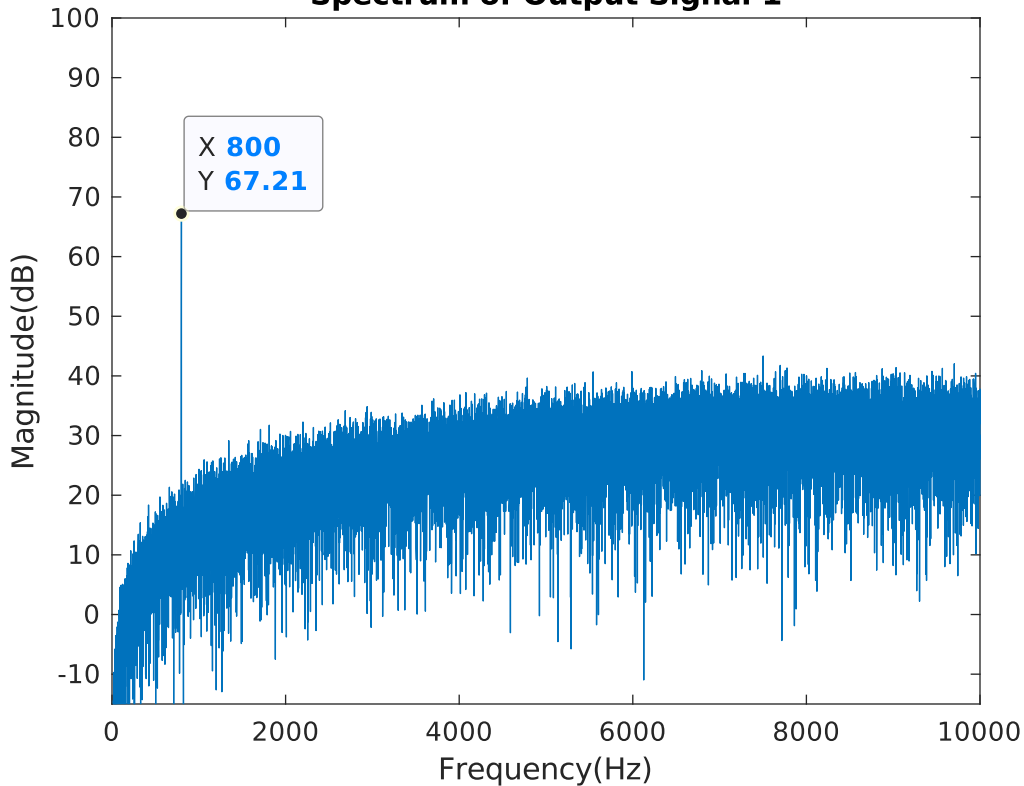
Spectrum of Output Signal 1
