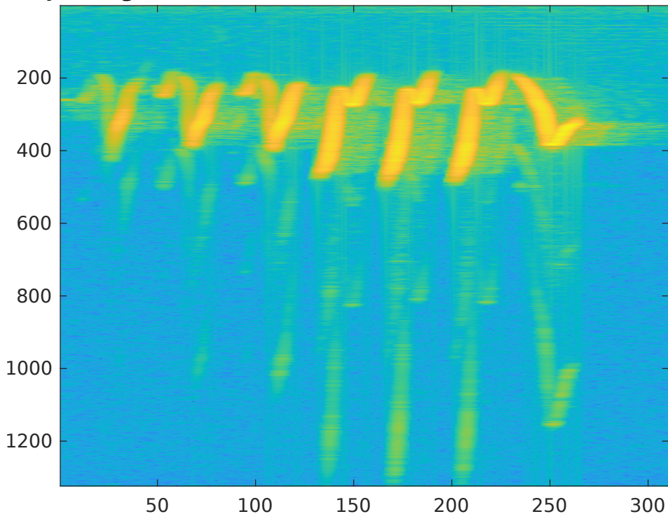
Spectrogram of sound.bird, Frame len. 60ms, Raw matrix
