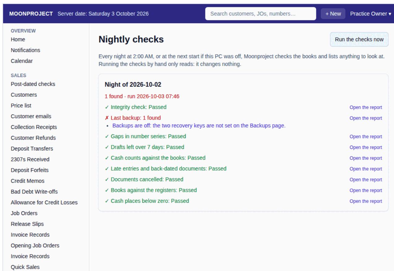
The Nightly checks screen · Owner-guide screenshot
