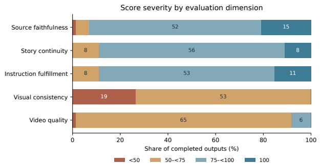
Figure 9 | Score distribution in the 72-output analysis sample.
