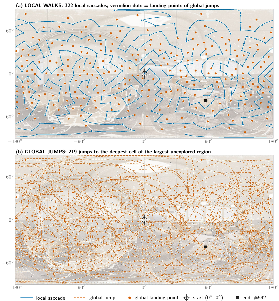
Figure 4: The complete 542-fixation gaze trajectory over the 360° sphere (CONTROLLER-TIME; gazes and decisions from the official run). Equirectangular, yaw left to right, pitch up. The background is the final reconstructed RGB panorama, lightened ( DERIVED ). (a) Local saccades (solid blue) form short walks that follow measured surface into unexplored territory. (b) Global jumps (dashed vermilion) carry the gaze to the middle of the largest remaining hole; late in the run, most of them land in small isolated holes. Grey dots in (b) are the other fixations.
