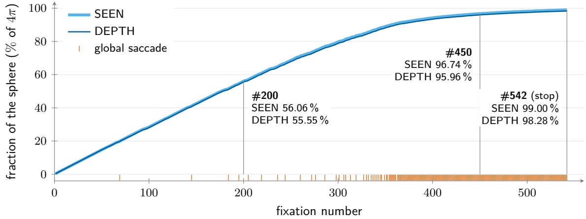
Figure 5: Growth of SEEN and DEPTH with fixation number (CONTROLLER-TIME, MEASURED, official run). Ticks along the bottom mark the 219 global saccades. The two curves nearly coincide because almost every direction that was looked at also returned depth. Three phases are visible: fast local exploration (few global jumps before #200); a mixed phase in which global jumps become frequent (#201–#450); and a long tail of single global jumps into small holes (#451–#542).
