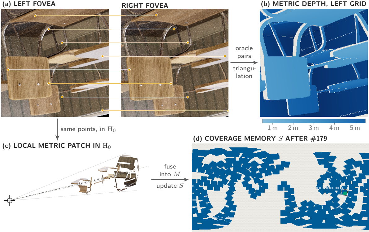
Figure 2: One fixation (#179, gaze yaw 130.0^\circ , pitch -9.3^\circ ). (a) The binocular foveal pair ( 256 \times 256 px each; 64-spp render, display RGB), with eight corresponding pixels, one per epipolar row. Corresponding points share a row, and their horizontal offset is the disparity. These are ORACLE correspondences, shown by reprojecting the triangulated points ( DERIVED ). (b) Range from the left eye on the left foveal grid ( DERIVED ); 0.5–5.5 m scale. (c) The fixation’s 60,778 metric points in H_0 , seen obliquely, with the head (crosshair), the gaze ray (dashed) and the 12^\circ core (grey lines) ( DERIVED ). (d) The cyclopean coverage after this fixation ( CONTROLLER-TIME ): DEPTH dark blue, SEEN light blue, UNSEEN stippled grey. Green marks the cells this fixation added; the black outline is its 12^\circ footprint. The fusion matched 36,481 points to existing surfels and created 24,297 new ones; the map grew to 8,836,458 surfels (MEASURED).
