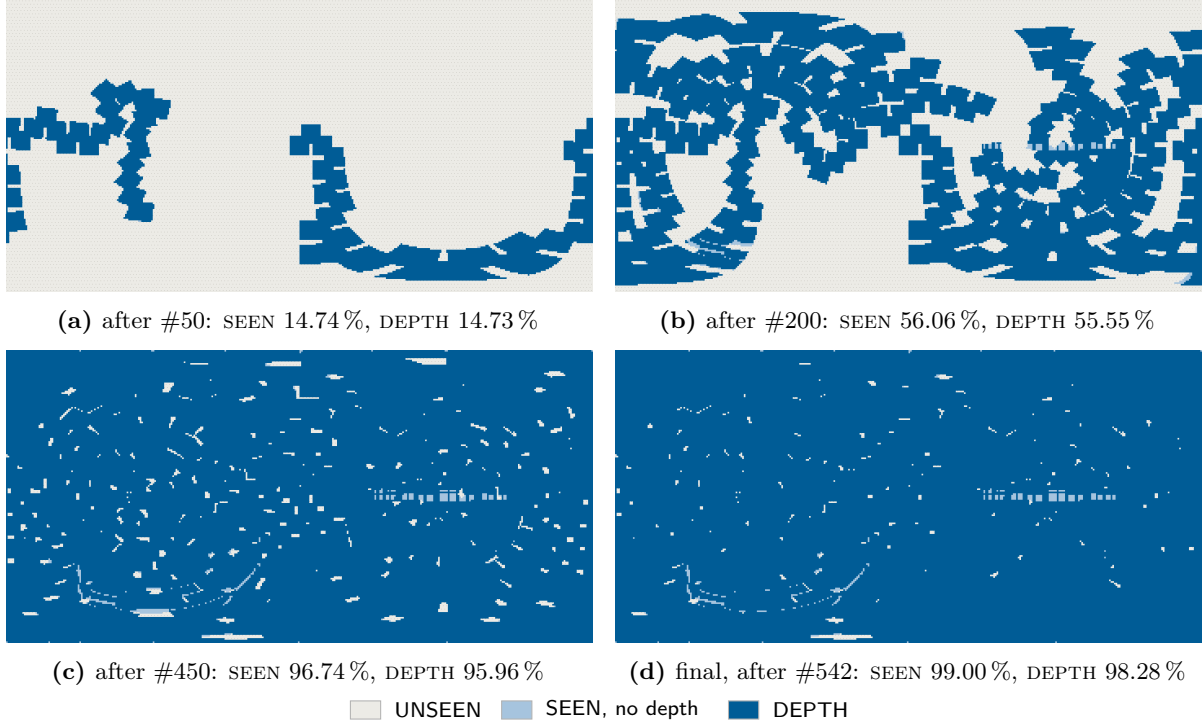
Figure 3: Cyclopean coverage memory at four stages (CONTROLLER-TIME; the state the policy actually used). Equirectangular, yaw -180^\circ \rightarrow +180^\circ from left to right, pitch +90^\circ at the top. Percentages are fractions of 4\pi (MEASURED, official run). The early walk covers contiguous regions. By #450 only scattered small holes remain, and the final state leaves 1.0 % UNSEEN in 184 small holes plus 0.72 % SEEN without depth (mostly the windows).
