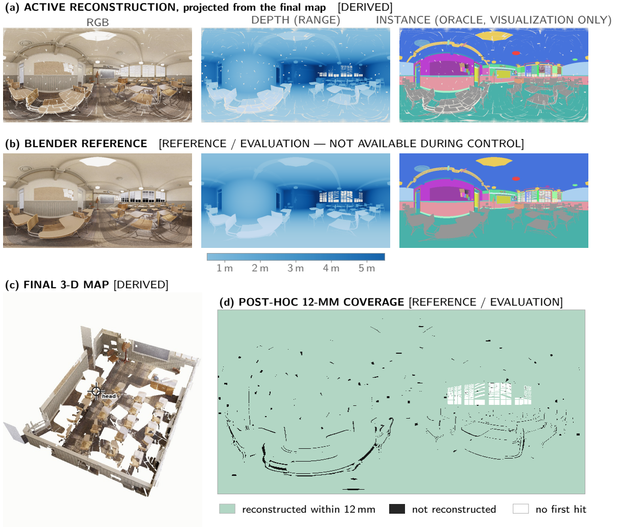
Figure 6: Final reconstruction and reference. (a) The final map projected onto the sphere from the head origin, nearest surfel per pixel: display RGB, range, and oracle instance labels ( DERIVED ; instance colours are ORACLE / VISUALIZATION ONLY and played no role in the run). Stippled grey = nothing reconstructed in that direction. (b) The independent Blender reference at 0.5^\circ ( REFERENCE / EVALUATION , never available during control). (c) The 16.5-million-surfel map seen from above and behind the head, with the ceiling removed for display ( DERIVED ). (d) Post-hoc evaluation over the reference sphere: 98.32% of the first-hit reference solid angle is reconstructed within 12mm. The misses are small holes and thin depth-edge slivers; the windows (white) have no first hit. Panels (a)–(c) are images from the frozen demonstration, whose control path the official reproduction matches bitwise.
