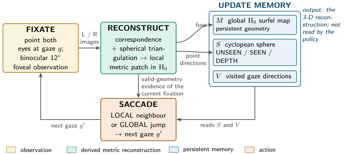
Figure 1: The Fixate–Reconstruct–Saccade loop. One fixation produces a binocular observation (orange), from which a local metric patch is derived (green). The patch is fused into the persistent map M , and its directions update the cyclopean coverage S (blue). The saccade decision (vermillion) reads only S , the visited directions V and the current fixation’s valid-geometry evidence. The map M is the system’s output; it is not fed back to gaze selection in this baseline.
