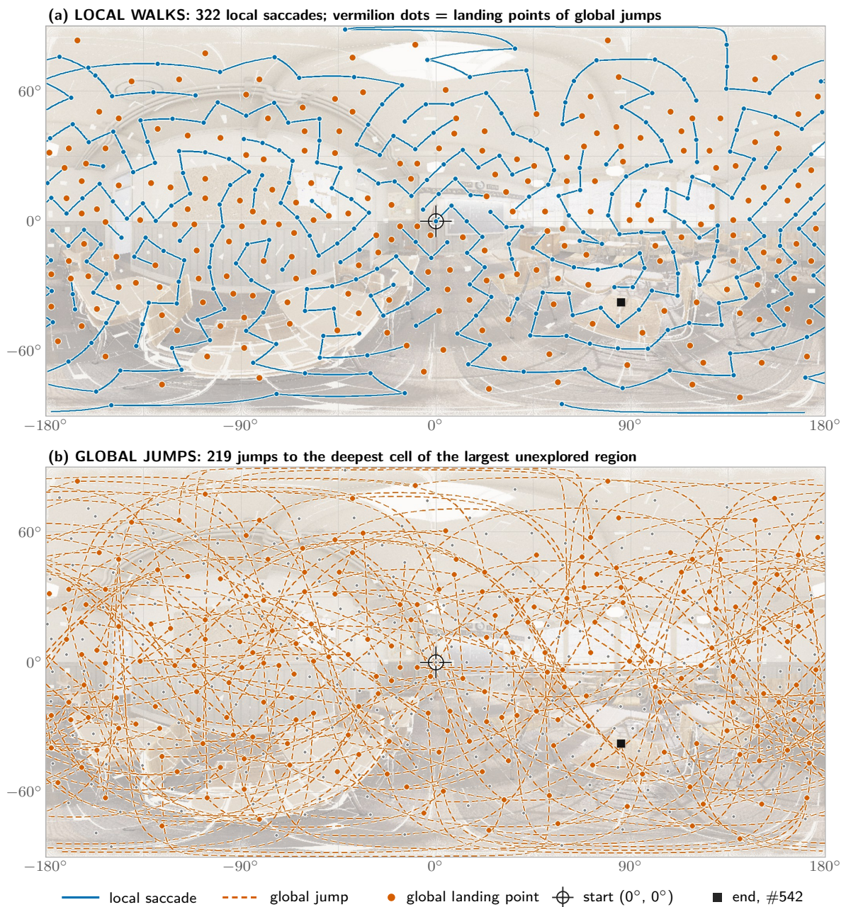
Figure 4: The complete 542-fixation gaze trajectory over the 360° sphere (CONTROLLER-TIME; gazes and decisions from the official run). Equirectangular, yaw left to right, pitch up. The background is the final reconstructed RGB panorama, lightened ( DERIVED ). (a) Local saccades (solid blue) form short walks that follow measured surface into unexplored territory. (b) Global jumps (dashed vermillion) carry the gaze to the middle of the largest remaining hole; late in the run, most of them land in small isolated holes. Grey dots in (b) are the other fixations.
