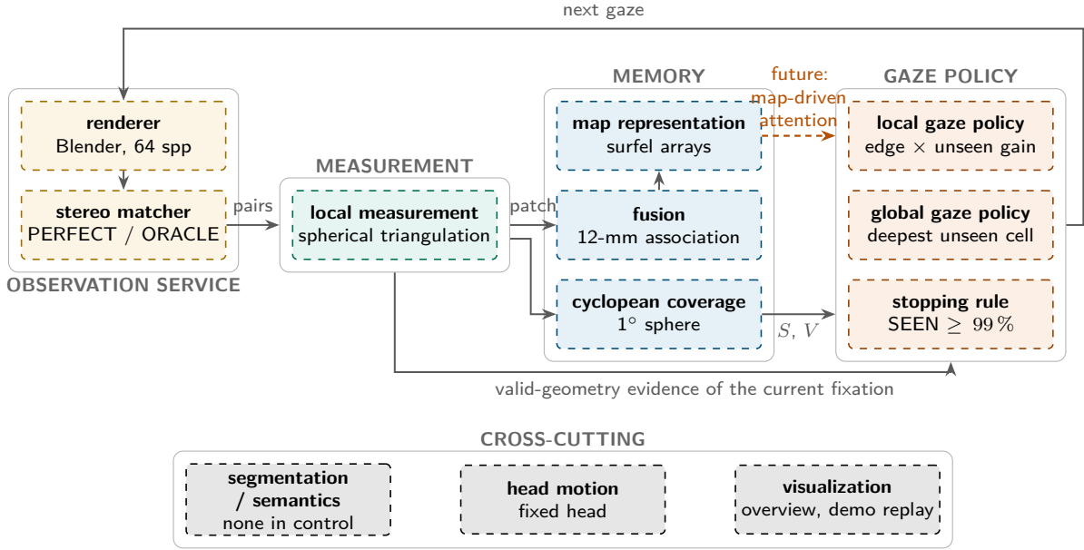
Figure 7: Playground extension map. Every dashed box is a replaceable component, coloured by role: observation (orange), measurement (green), memory (blue), gaze policy (vermilion), cross-cutting (grey). Solid arrows are the data flow of the baseline. The dashed vermilion arrow from the map to the policy is not part of the baseline: map-driven attention is a future experiment, and in the baseline the policy reads coverage, visited directions and the current fixation’s evidence only.
