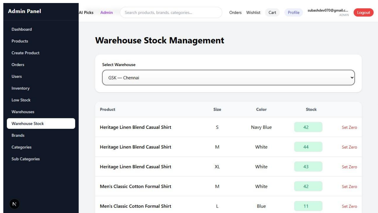
Fig:5.3.11 Warehouse Stock Management Interface
