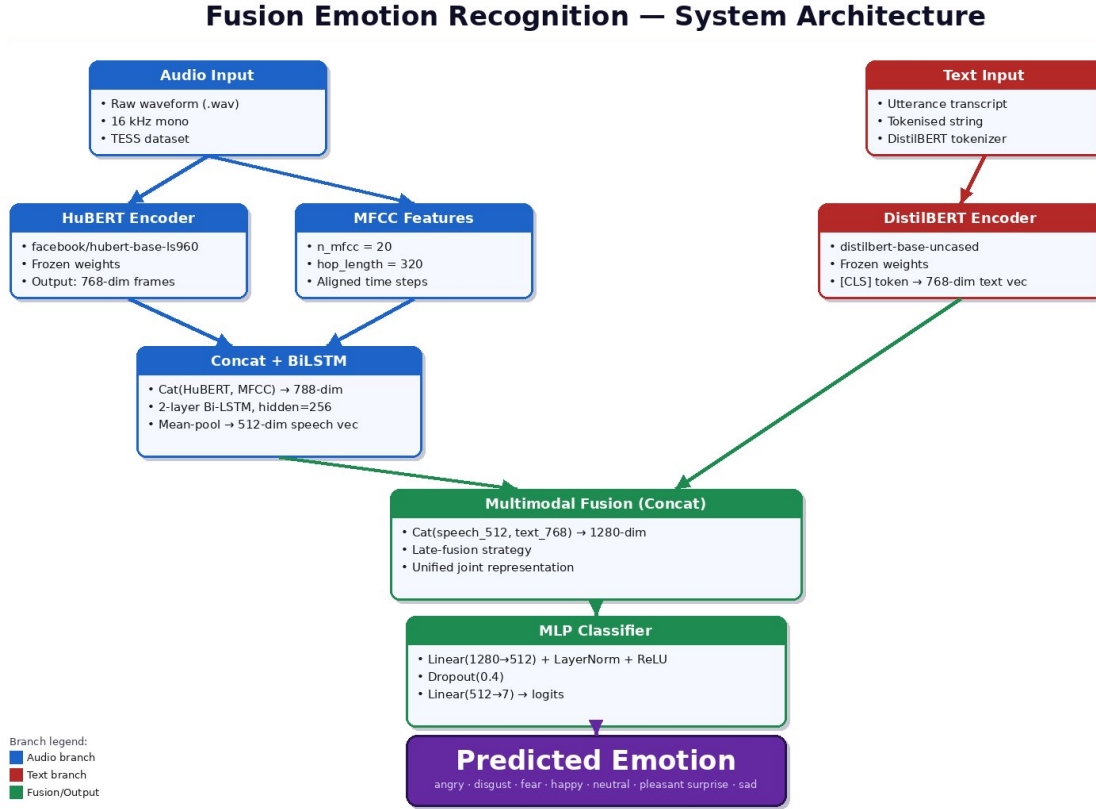
Figure 5.3: Multimodal Fusion Emotion Recognition System Architecture
