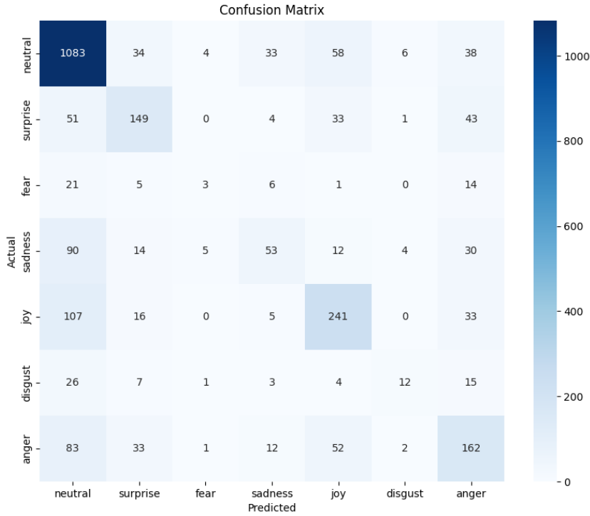
Figure 7.6: Confusion Matrix for the MELD Text Emotion Recognition Model
