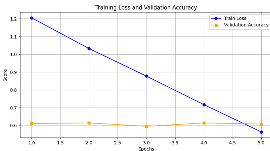
Figure 7.5: Training Loss and Validation Accuracy Curves for the MELD Model
