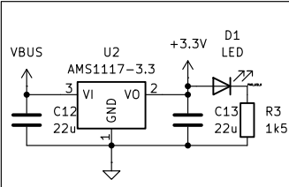
Power Supply
