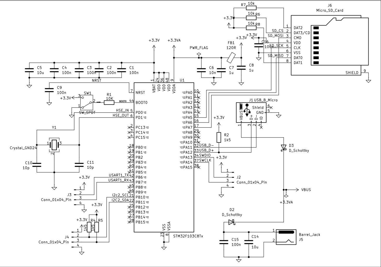
Microcontroller (and USB)
