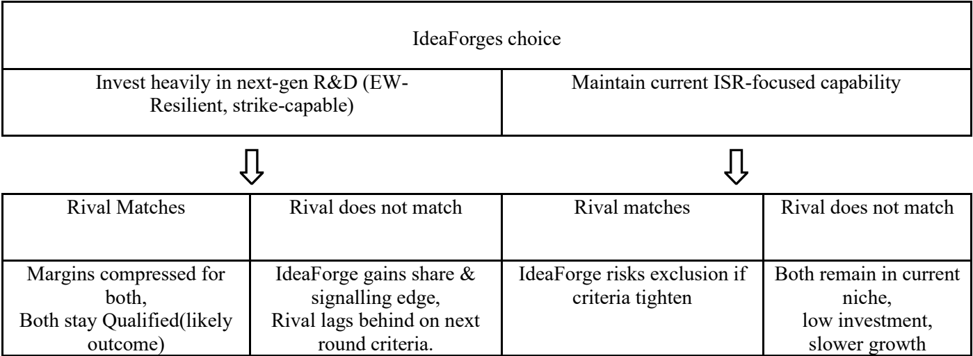
Payoff matrix: IdeaForge, Rival
