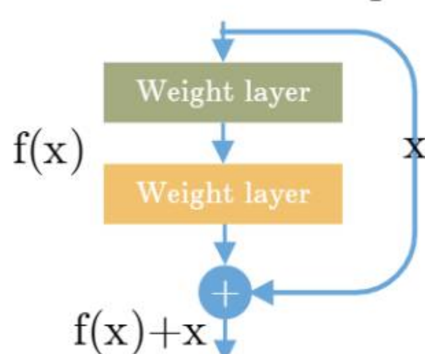
Figure 1 ResNet Block
