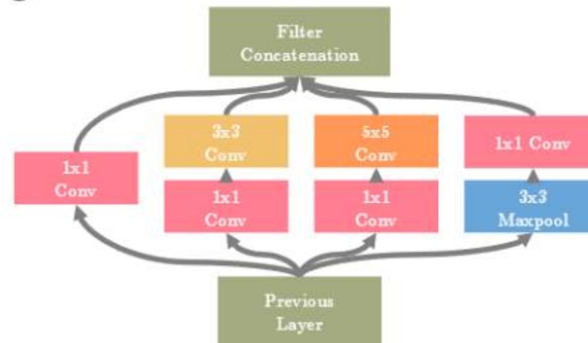
Figure 2 Inception Block
