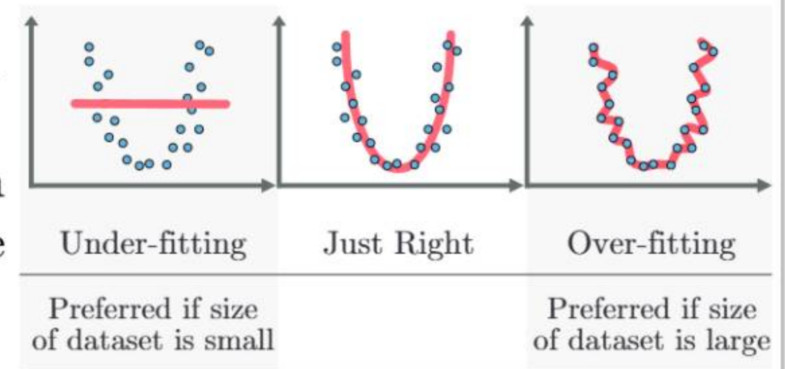
Figure 1. Overfitting
