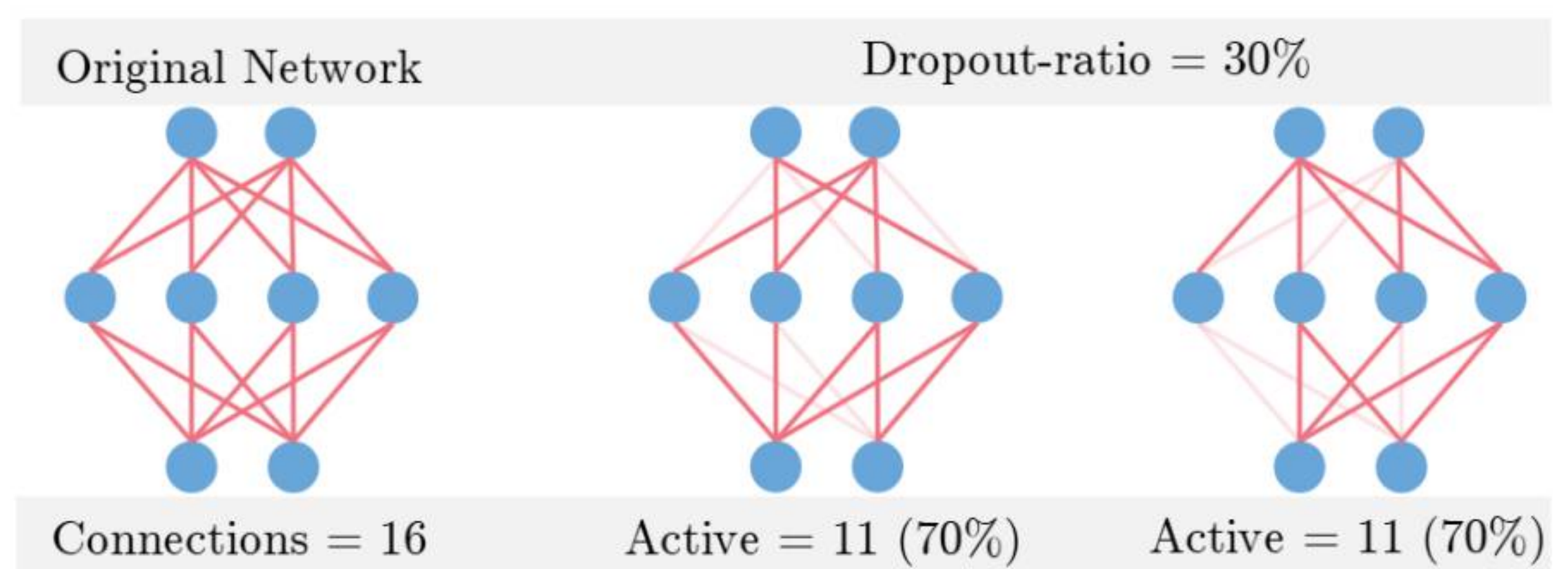
Figure 3. Drop-out
