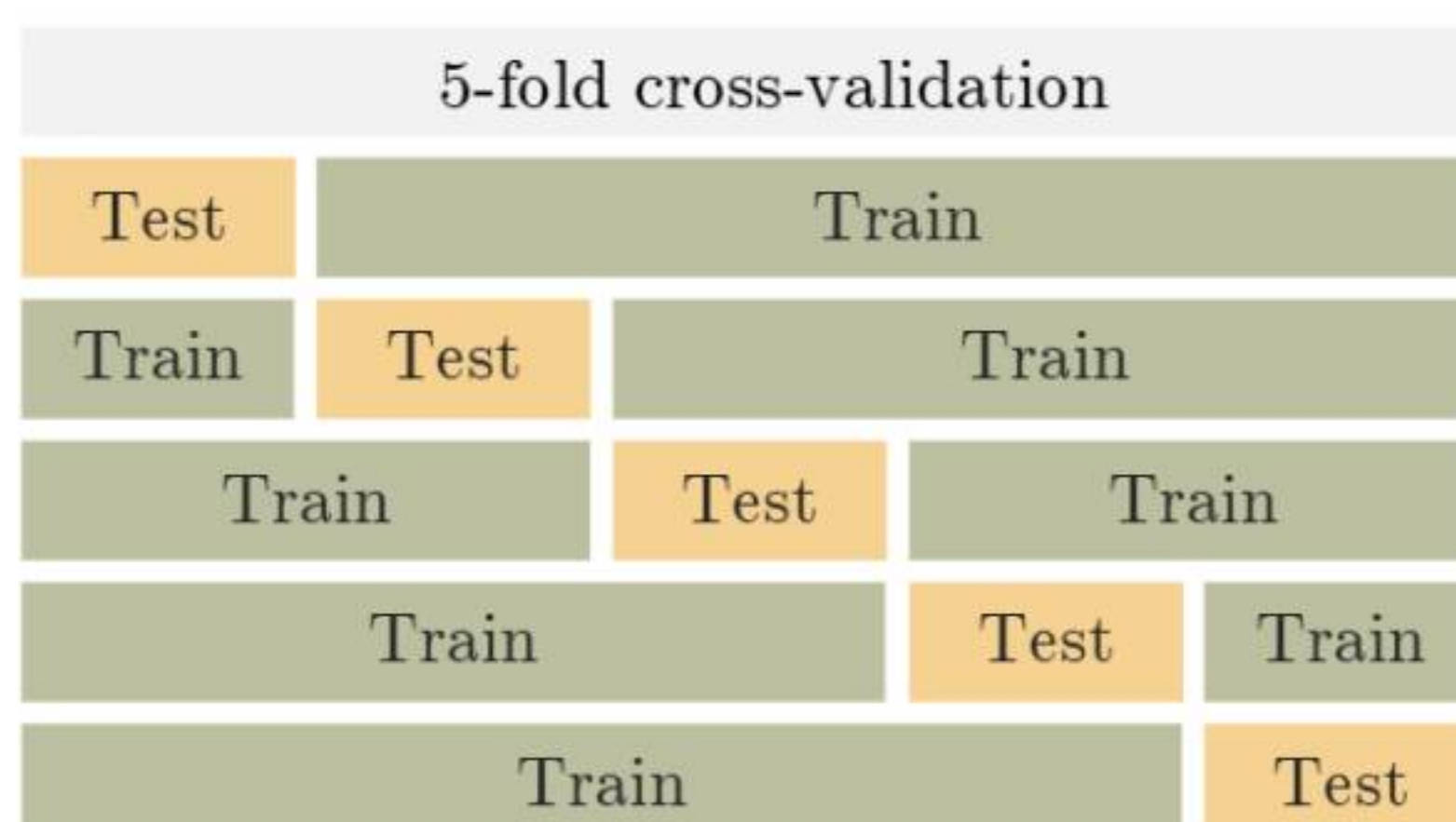
Figure 2. K-fold CV
