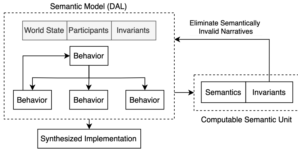
Figure 7: Computable Semantic Model
