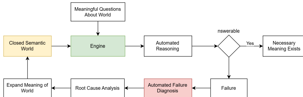
Figure 15: Establish necessary meaning by answering meaningful questions through semantic reasoning.
