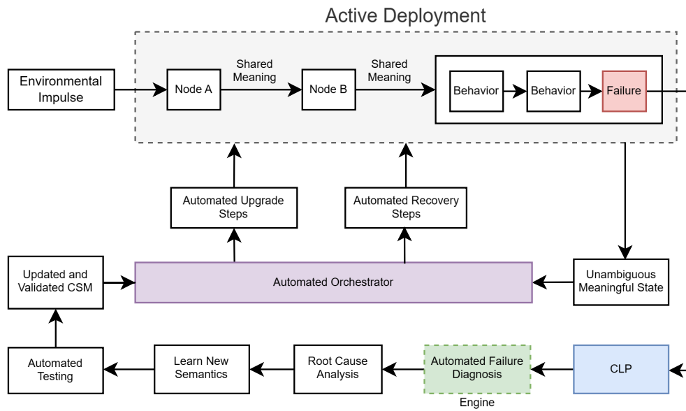
Figure 14: Automated Orchestration of Recovery from Mechanical Failures
